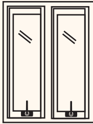
L-Top Hung R-Top Hung + Center Mullion
