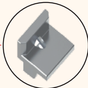
Euro Striker: Receives locking bolt for secure multi point locking
