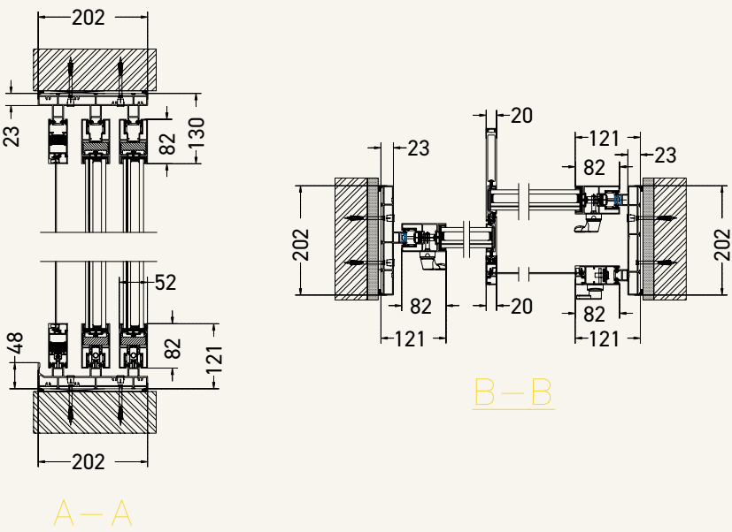
Cross Section
