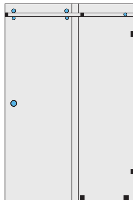
1 FIXED GLASS + 1 SLIDING DOOR (RIGHT SLIDING)
