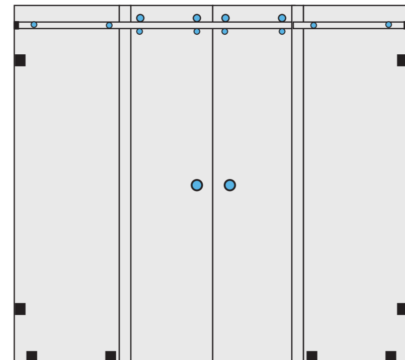
2 FIXED GLASS + 2 SLIDING DOORS
