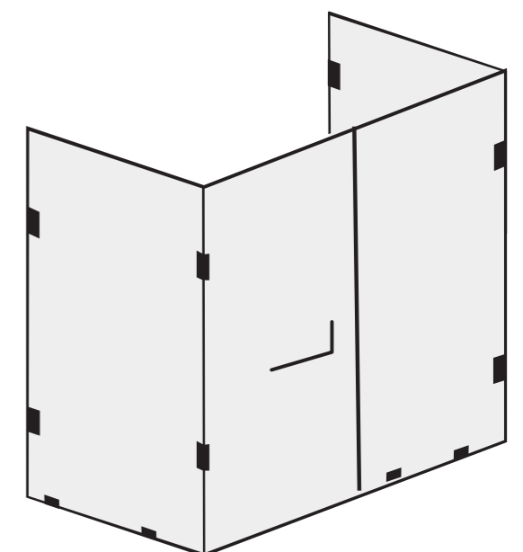
1 LEFT DOOR+ 3 FIXED GLASS (WITH 90° GLASS TO GLASS HINGE) C SHAPE
