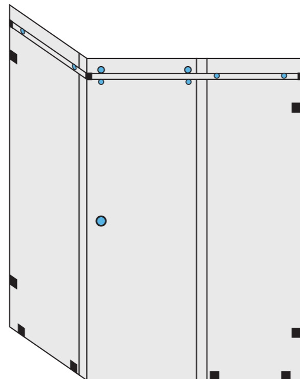
2 FIXED GLASS + 1 RIGHT SLIDING DOOR (90° WALL)
