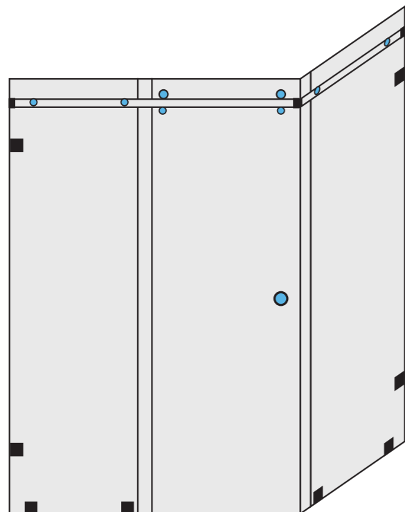
2 FIXED GLASS + 1 LEFT SLIDING DOOR (90° WALL)
